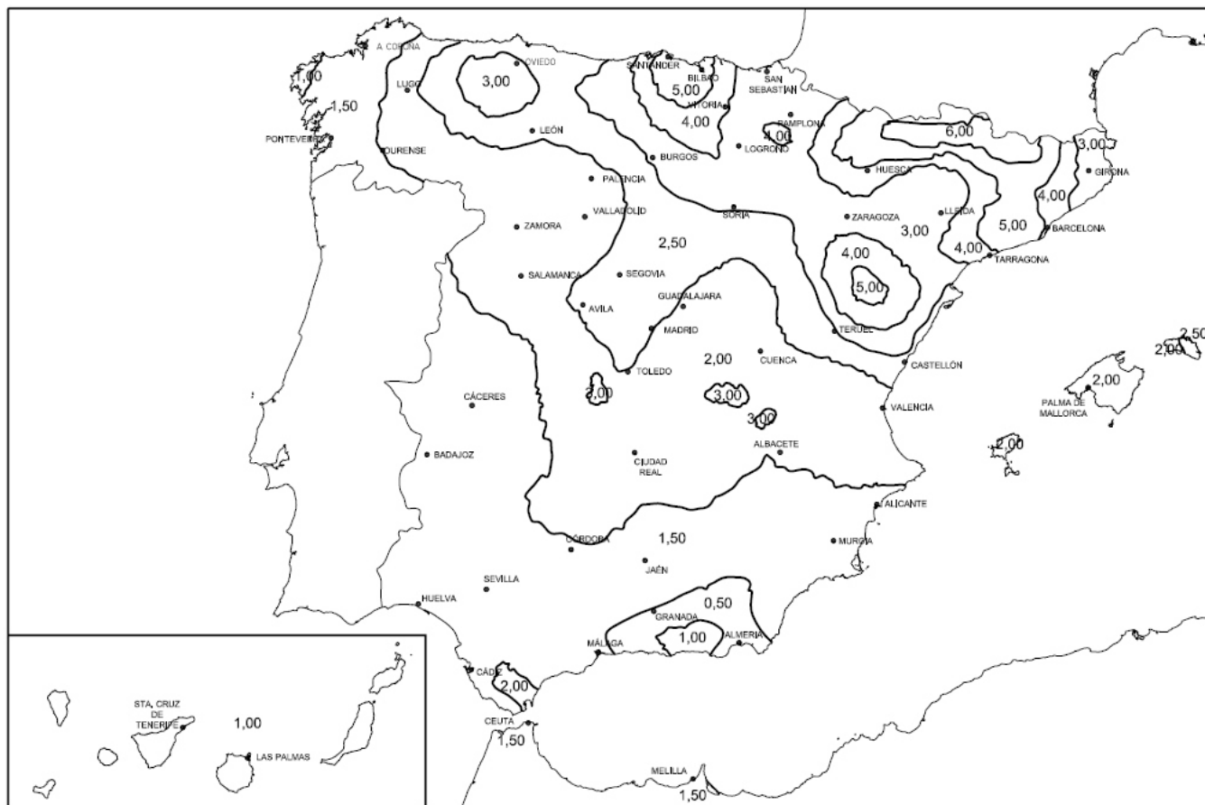
Figure B.2 – Map of Ng level for Spain
