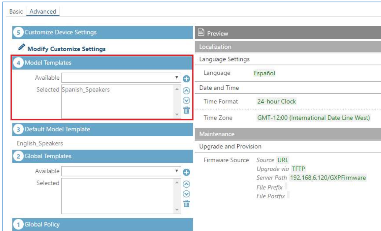
Figure 84: Zero Config Sample - Device Preview 2
