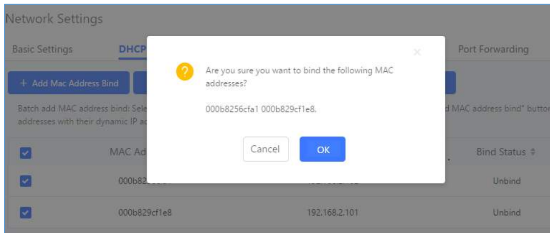
Figure 17: Batch Add MAC Address Bind
