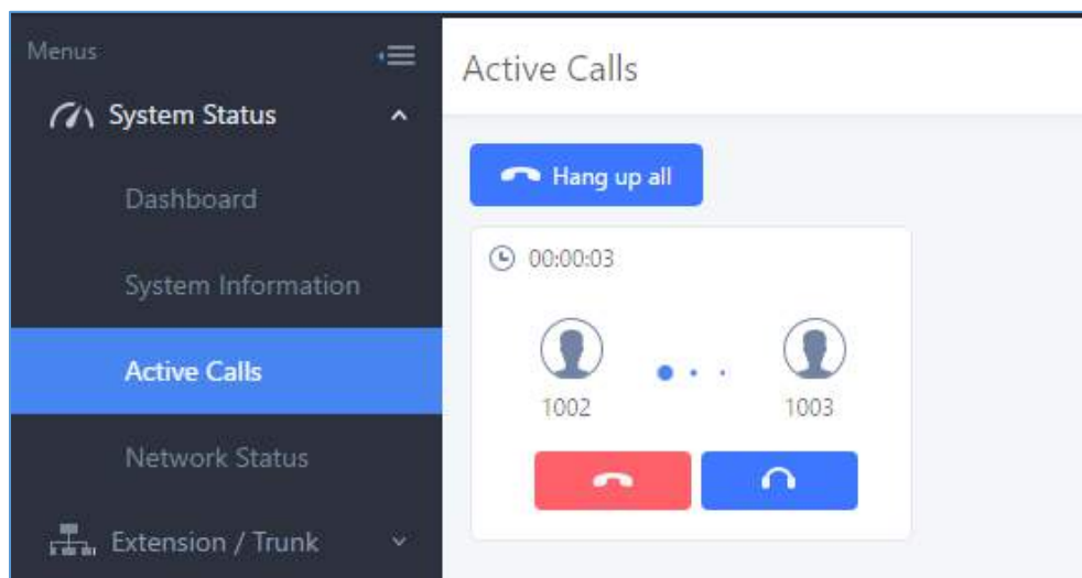
Figure 185: Status→PBX Status→Active Calls – Call Established
