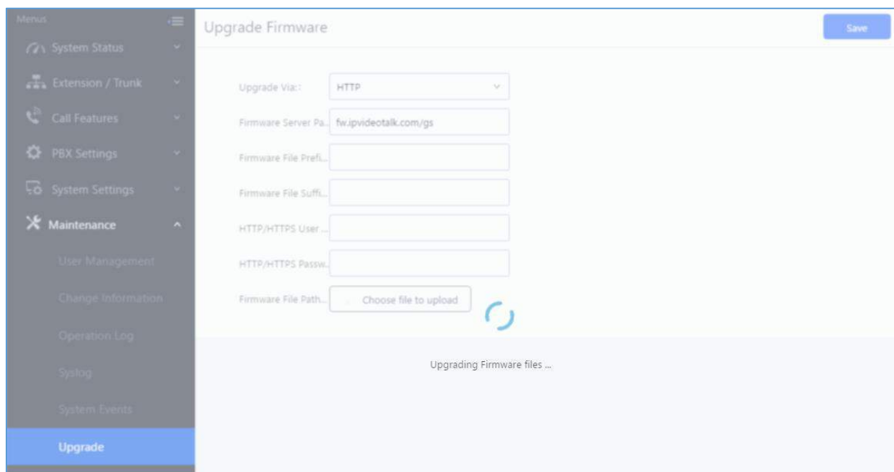
Figure 271: Upgrading Firmware Files
