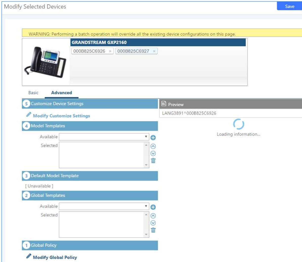
Figure 79: Modify Selected Devices - Same Model
