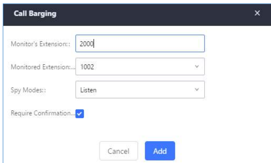
Figure 189: Configure to Monitor an Active Call
