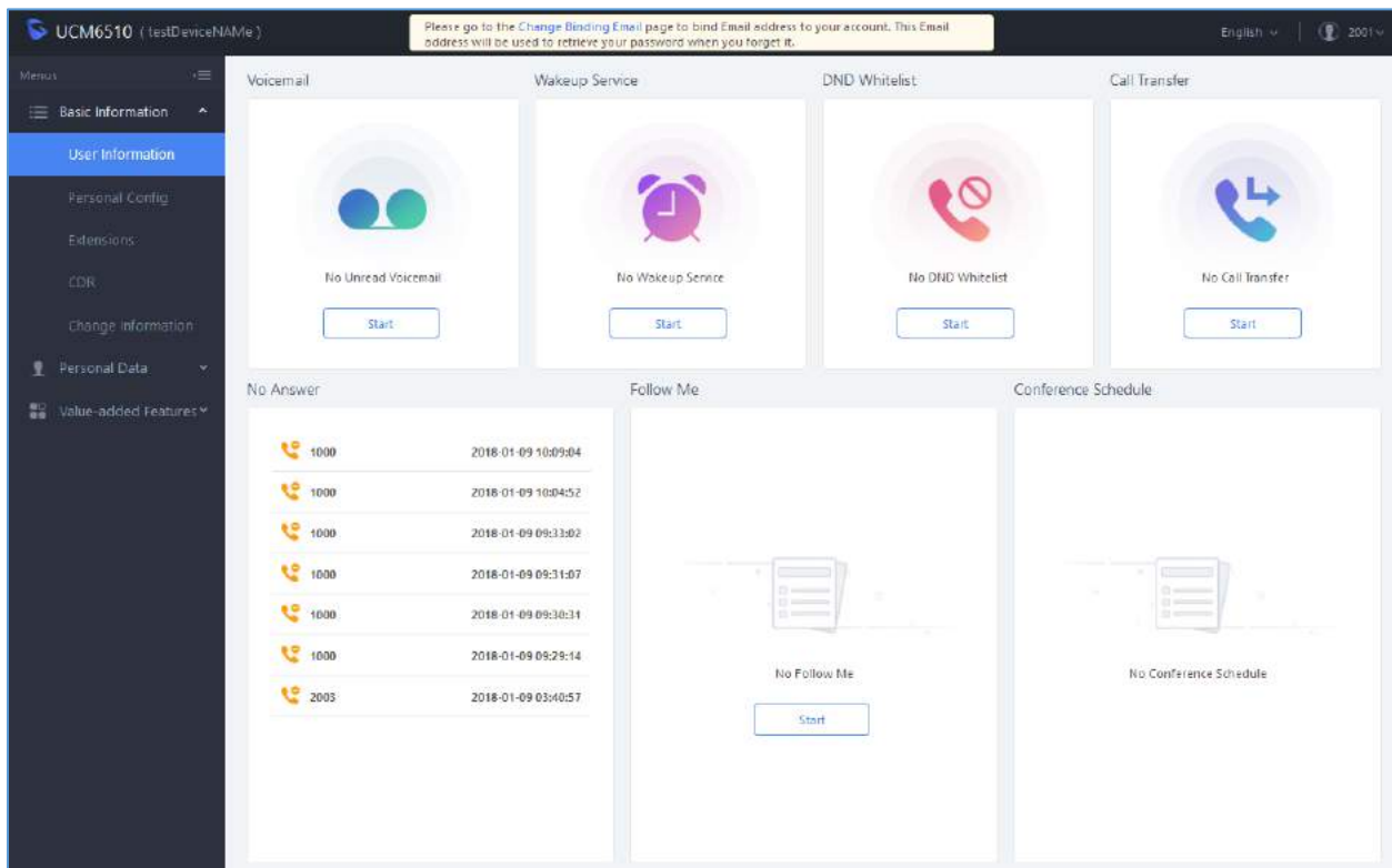
Figure 256: User Portal Layout
