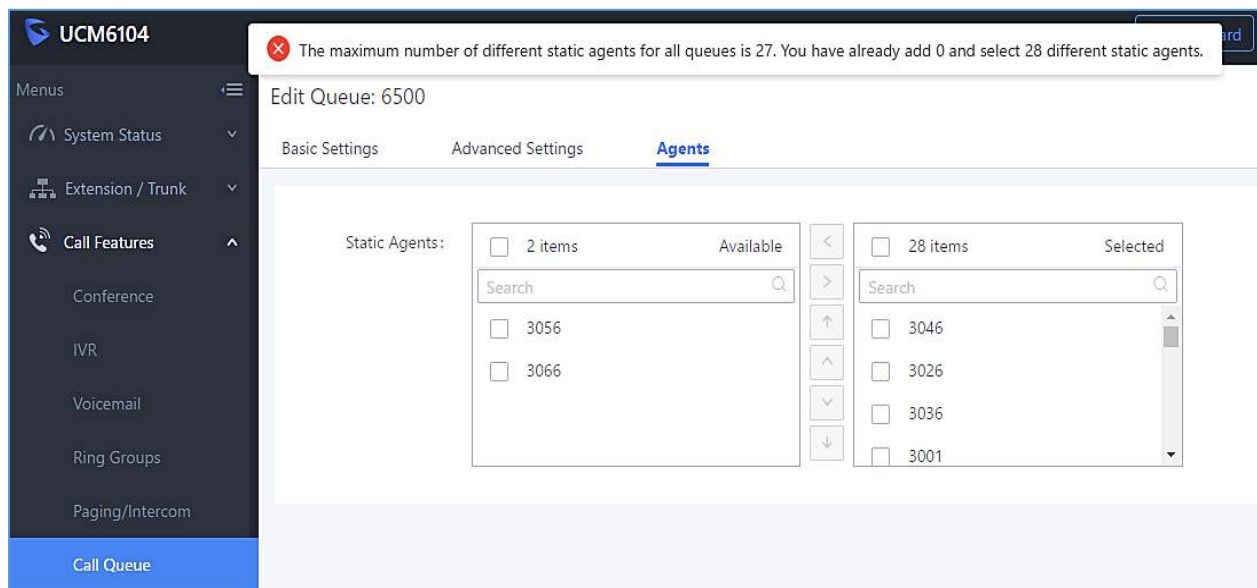
Figure 149: Static Agents limitation
