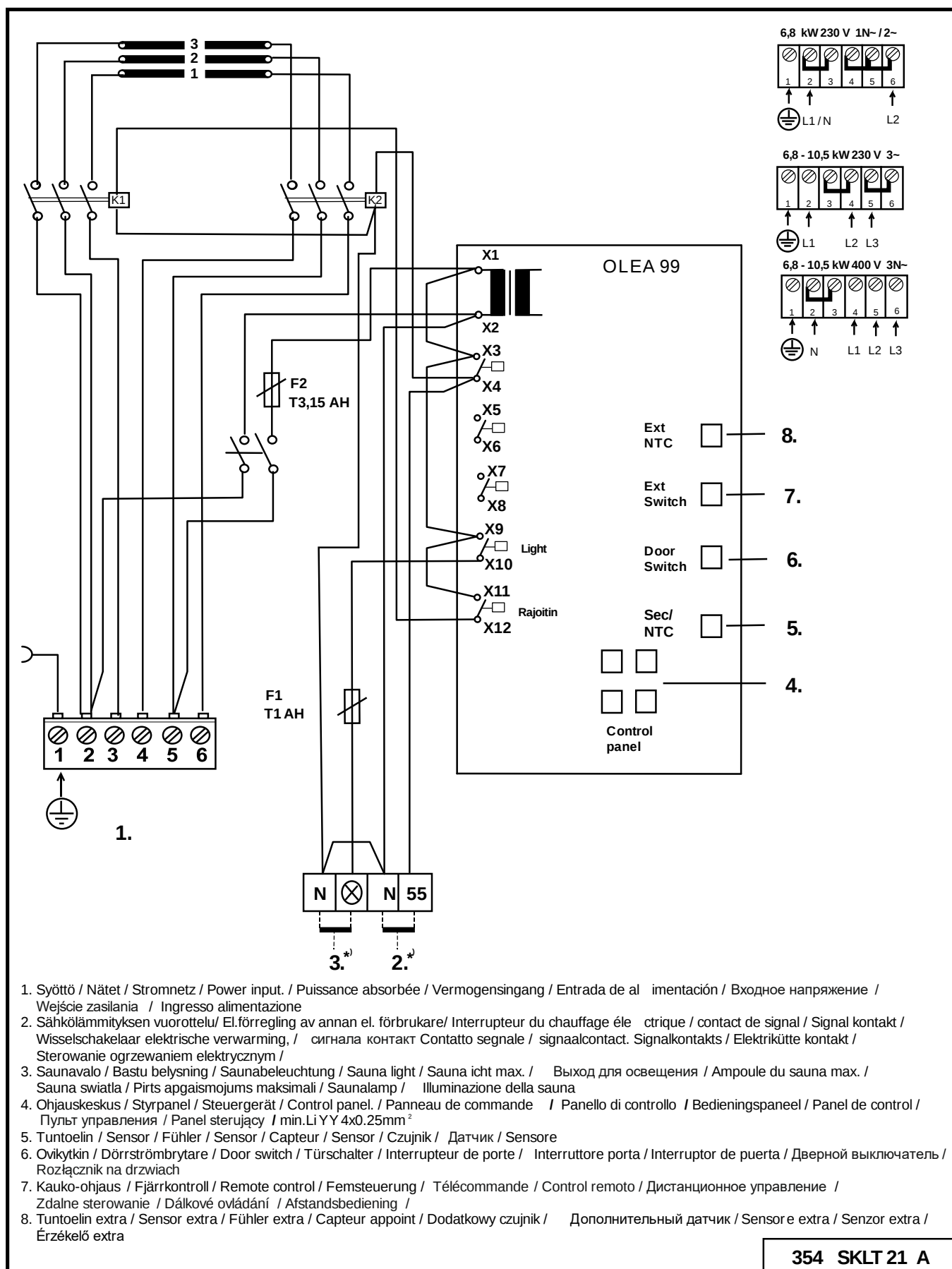
Figure 7 Wiring diagram for the sauna heater
