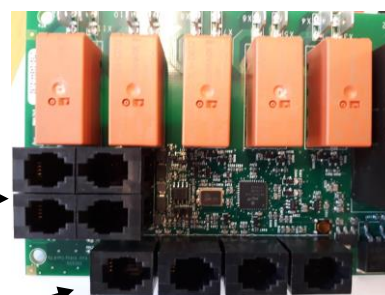
Figure 4 . Order of RJ 10 connectors. Sensor, Door switch, Remote control, Additional NTC
