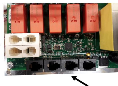
Figure 5 . Order of RJ 10 connectors. Sensor, Door switch, Remote control, Additional NTC
