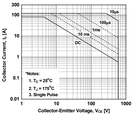
Figure 11. SOA Characteristics
