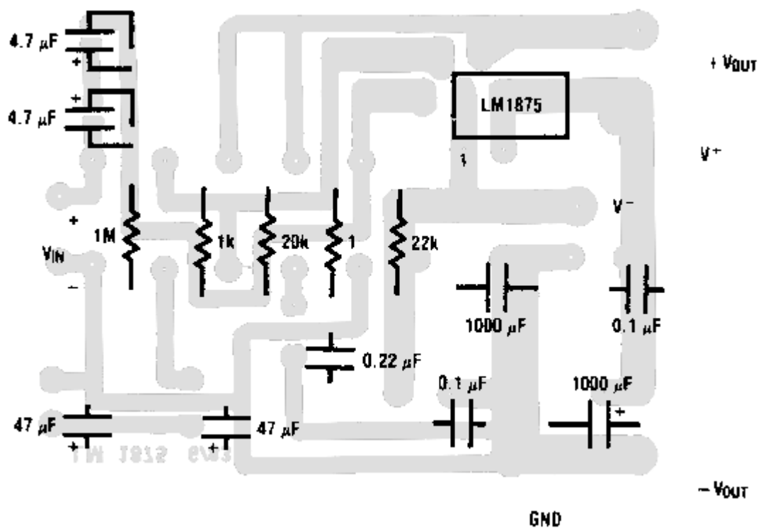
Figure 3. Split Supply
