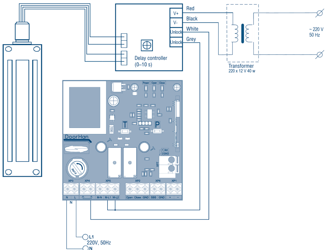
Fig. 4. Connection of electromagnetic lock
