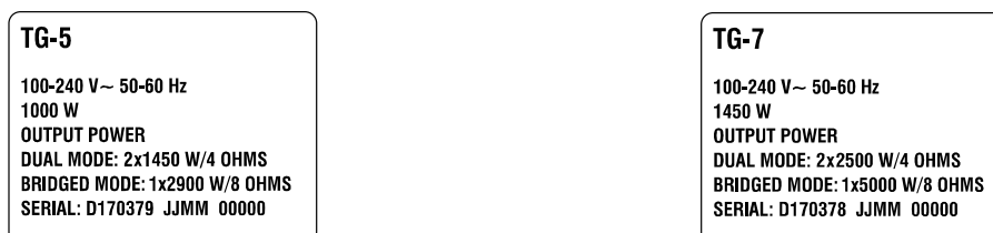
Illustration 2.3: TG-5/TG-7 type plate
