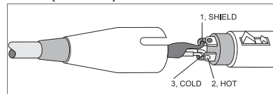
XLR (female)
