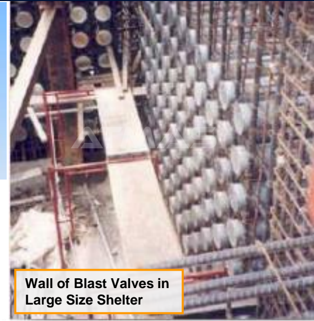
Automated blast gates
