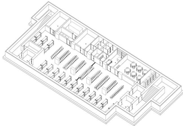
Design project of shelter for 250 people
