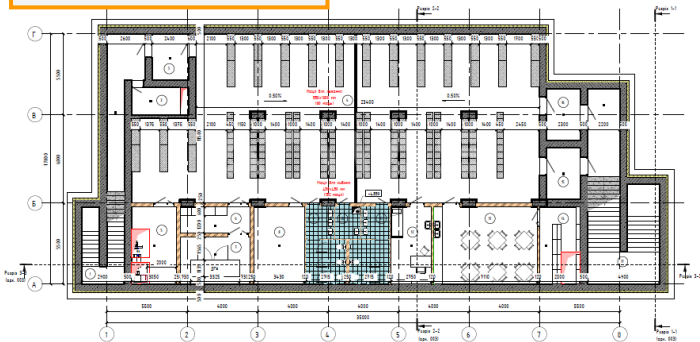
Design project of shelter for 250 people
