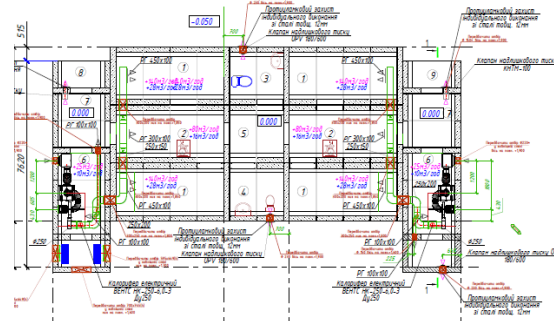
Design project of ventilation systems in the shelter
