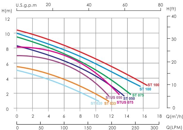
Remark: The performance curve above is for 50Hz models
