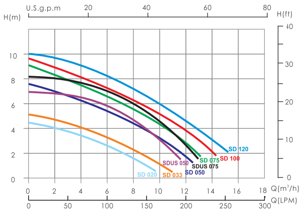
Note: The performance curve above is for 50Hz models
