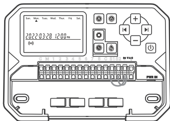
Smart Sprinkler Controller
