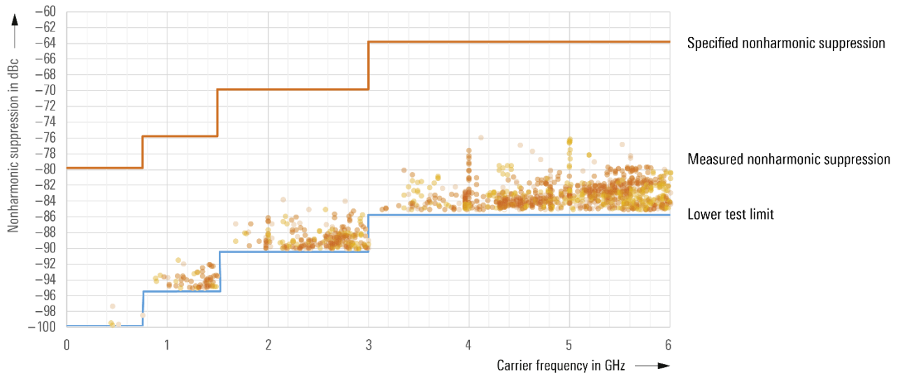
Spurious emissions (CW, carrier offset > 10 kHz) – several R&S®SMBV100B instruments measured
