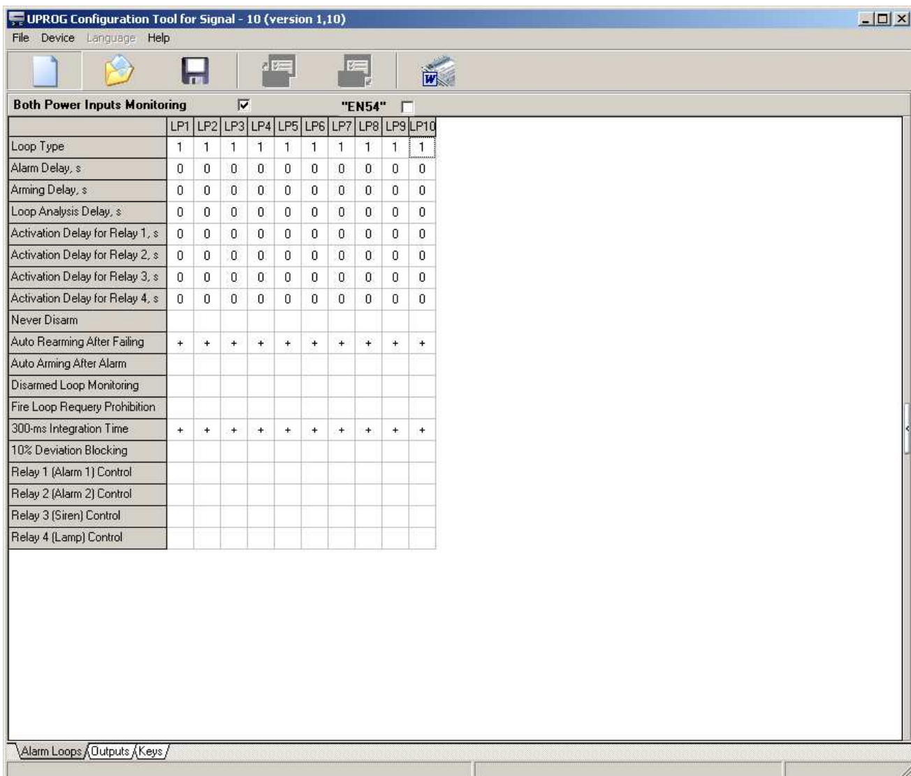
Figure 11. UProg Work Window for Configuring the Signal-10
