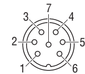
Front side molded 7P Male connector
