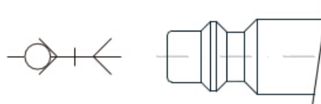
Profile ISO 6150 B12
