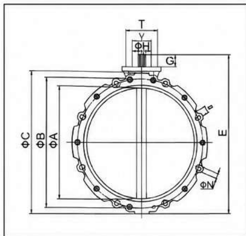
BV2F双法兰蝴蝶阀 Double flanged butterfly valve
