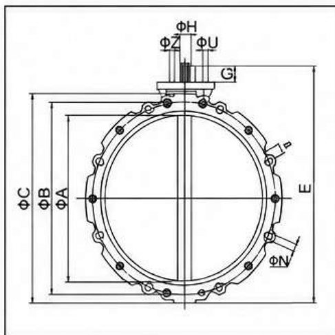
BV2F双法兰蝴蝶阀 Double flanged butterfly valve
