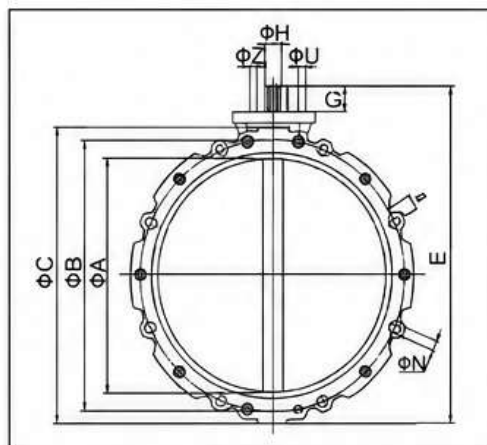
BV1F单法兰蝴蝶阀 single flanged butterfly valve
