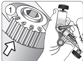
Set the jig, JS.
