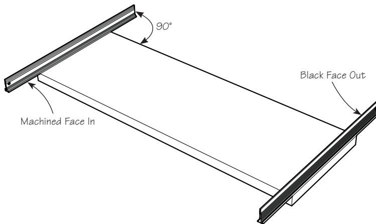
Figure 1: Setting up the winding sticks on a workpiece.
