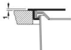
Surface mounting
